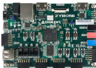
Digilent Zybo Z7 Development Kit
